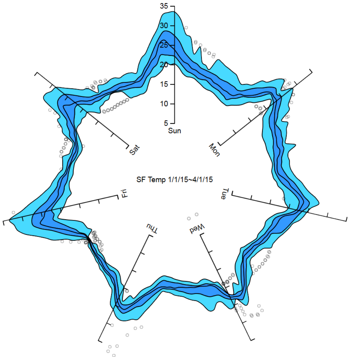
Figure 4.21: Example of Radial boxplot . Figure taken from the work of David Lin [Lin18]
