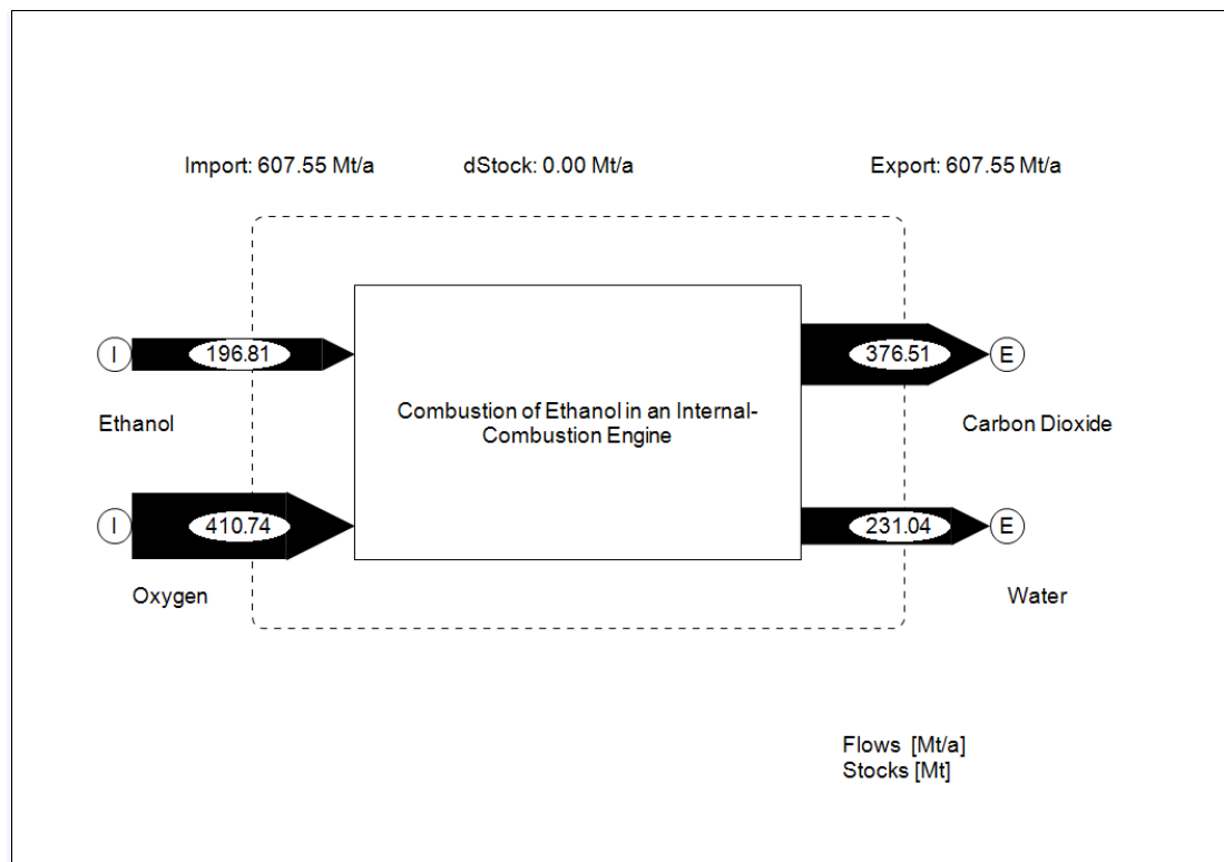
Figure 17: CO 2 Emissions from the Use of Ethanol in Cars in the U.S., 2010 (Source: author)
