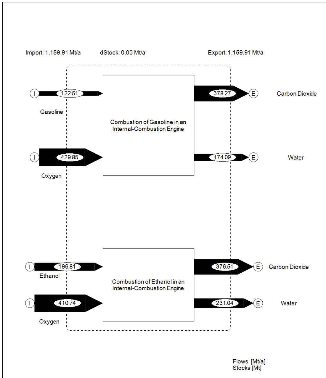
Figure 18: Comparison of the CO 2 Emissions from Gasoline and Ethanol in the U.S., 2010 (Source: author)
