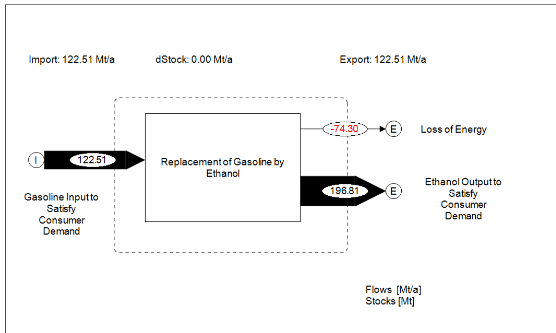
Figure 16: Replacement of Gasoline by Ethanol in the U.S., 2010 (Source: author)
