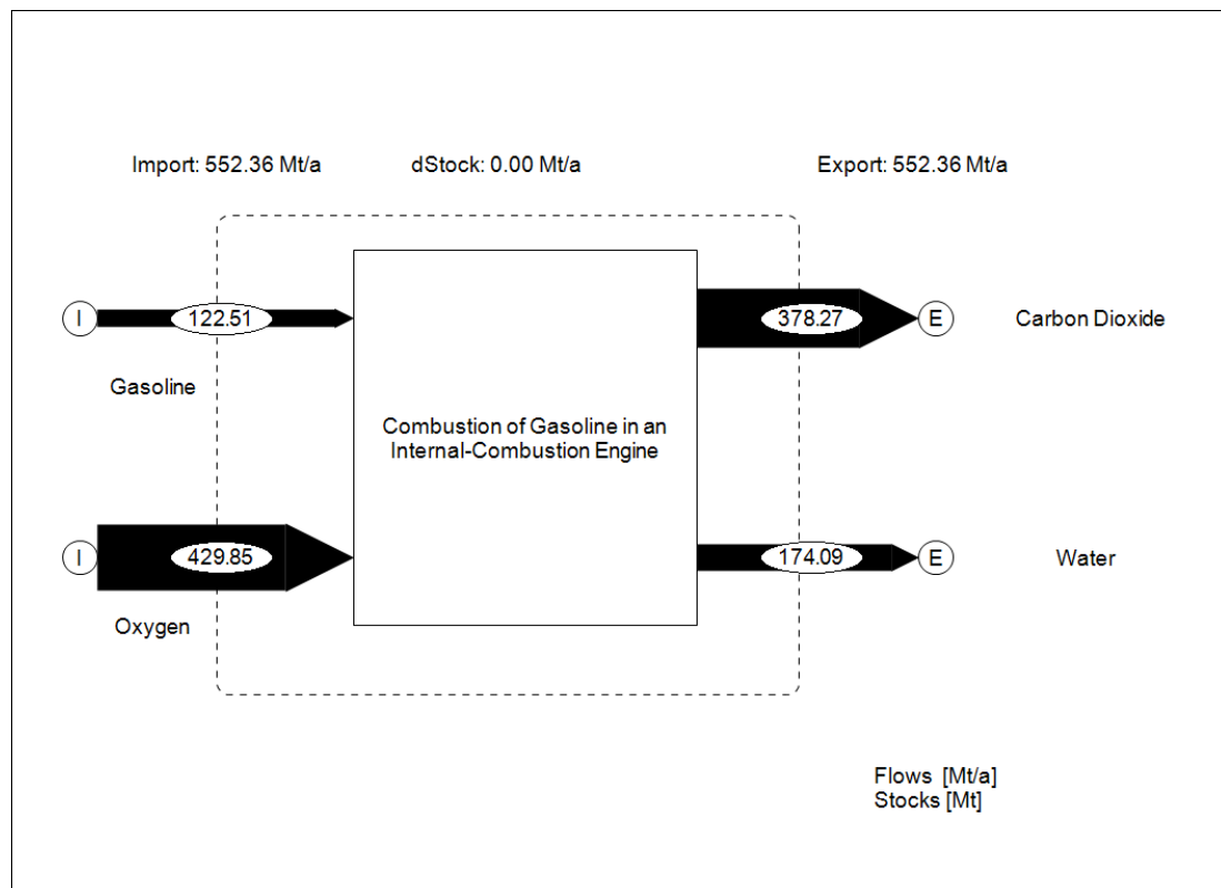
Figure 15: CO 2 Emissions from the Use of Gasoline in Cars in the U.S., 2010 (Source: author)
