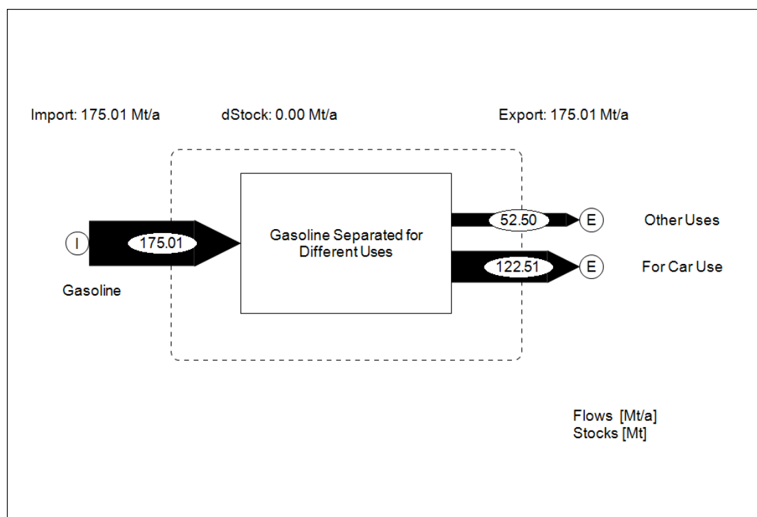
Figure 14: Gasoline Separated for Different Uses in the U.S., 2010 (Source: author)
