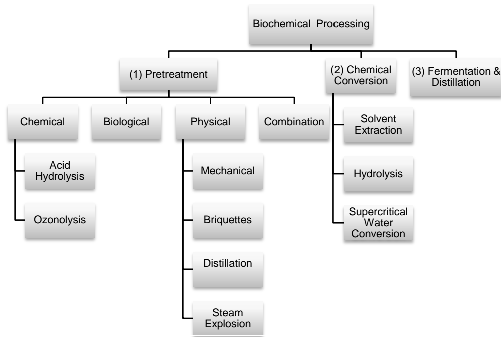
Figure 9: Summary of the Biochemical Processing of Lignocellulosic Biomass (Source: author)
