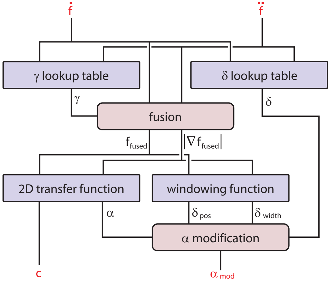
Figure 3.4: Overview over the processing steps for each sample point during the rendering process. Nodes with rounded corners are calculation steps and nodes with sharp corners are lookups.
