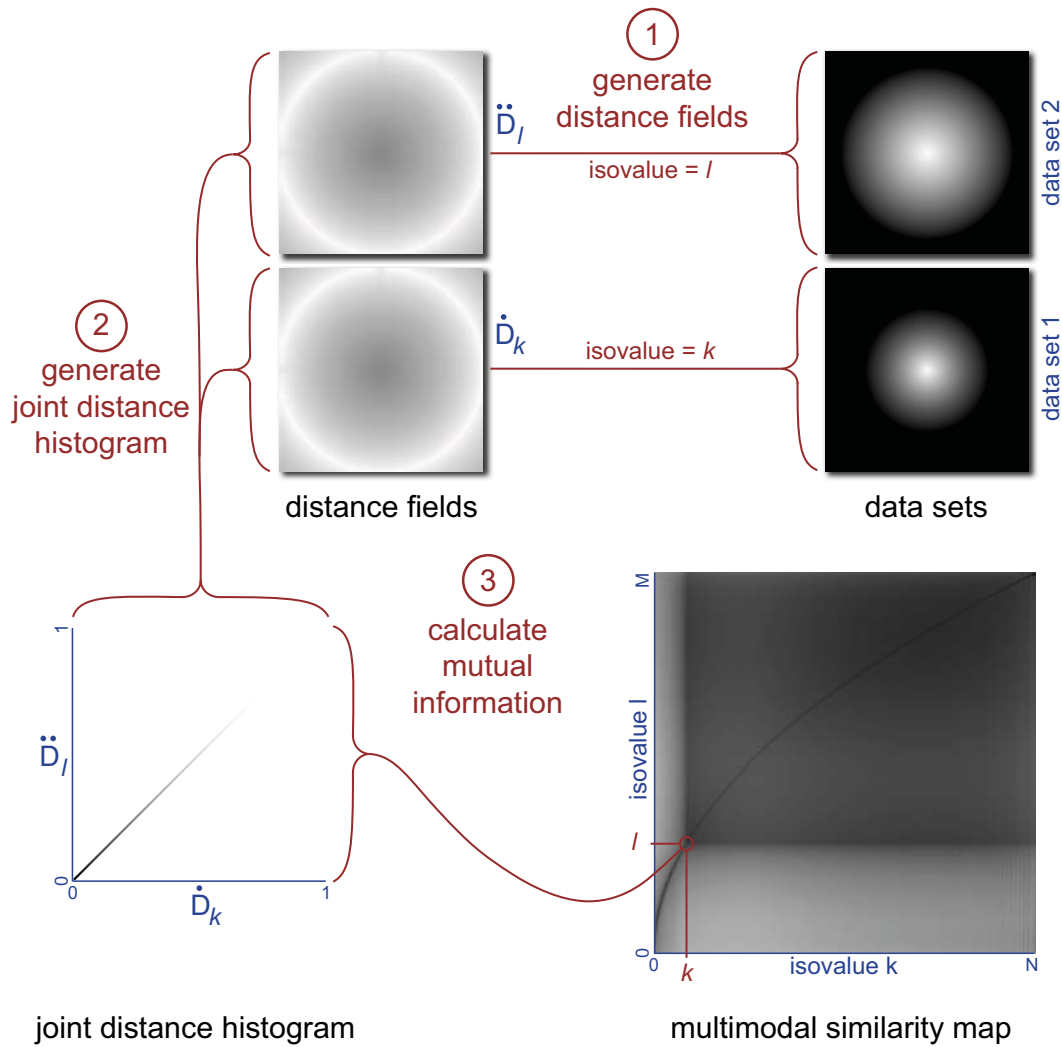
Figure 4.3: Pipeline for the generation of a multimodal similarity map. The illustration shows which steps are necessary to calculate the similarity of isosurfaces for the isovalue k and l .
