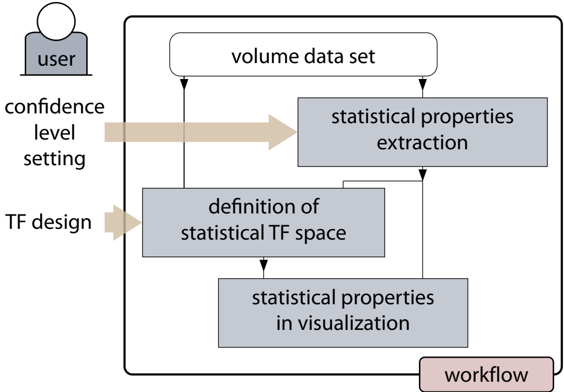
Figure 2.1: Statistical transfer-function workflow.
