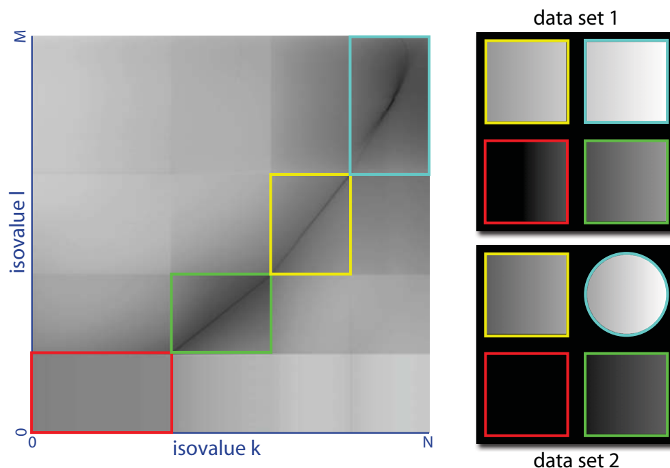
Figure 4.5: Multimodal similarity map for contradictory complementary data.
