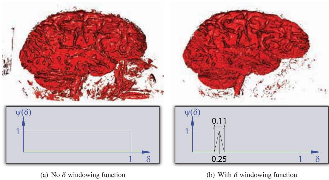
Figure 3.6: The two results show the effect of the usage of \delta to modify the optical properties of a 2D region in the transfer-function space.
