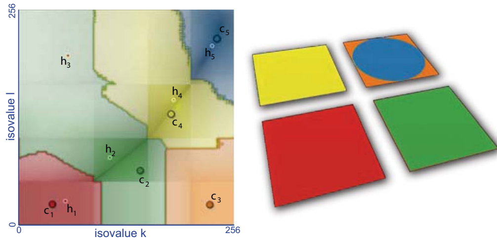
Figure 4.10: Classification based on multimodal similarity for complementary data.
