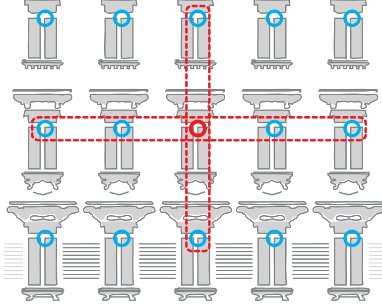
Figure 6.3.: Symmetry Neighborhood. Blue circles denote symmetry neighbors of the red one.
