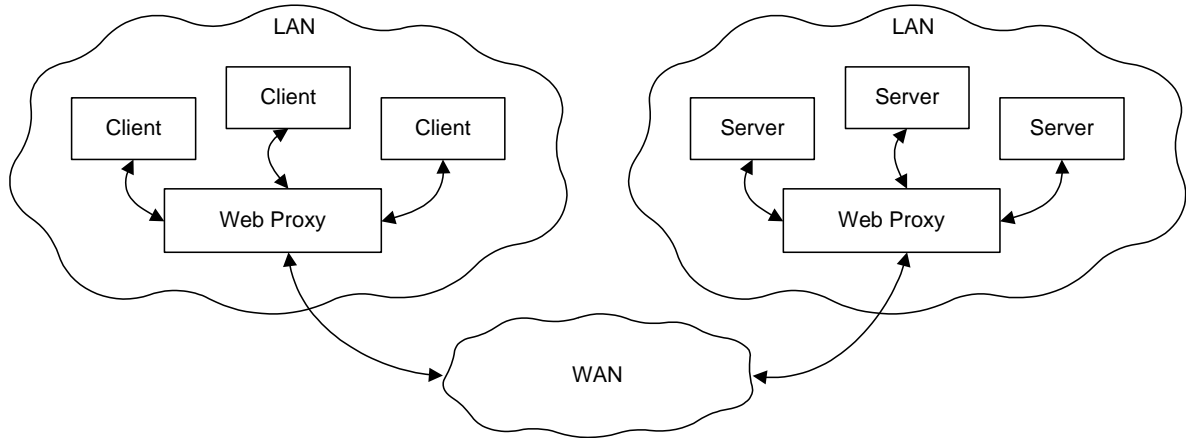
Figure 4.2: Using the WEB PROXY pattern
