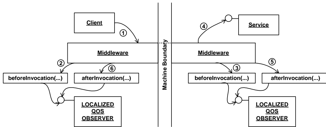
Figure 4.16: LOCALIZED QOS OBSERVER
