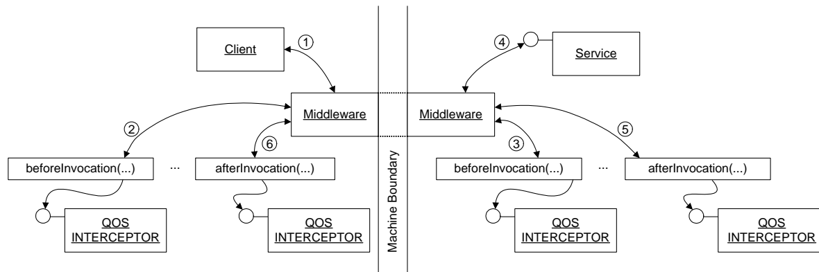
Figure 4.9: The QOS INTERCEPTOR pattern
