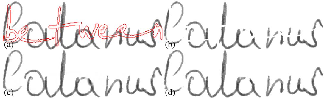
Figure 4.25: Inpainting of an overwritten area (Occlusion ratio: 10.6 %, mask width: 4.35 pixels) (a) Inpainting problem. (b) Background filling result (PSNR = 13.77 dB). (c) FOE result (PSNR = 21.72 dB). (d) Tensor voting result (PSNR = 19.69 dB).
