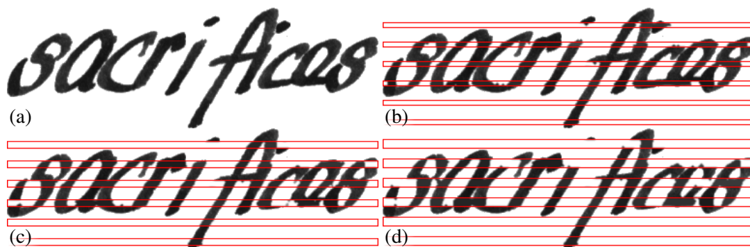
Figure 4.22: Restoring regions that are occluded by ruling lines. (a) Ground truth image. (b) 3 pixels wide ruling lines. \sigma = 3 : 17.79 dB. (c) 5 pixels wide ruling lines. \sigma = 4 : 14.55 dB. (d) 7 pixels wide ruling lines. \sigma = 7 : 12.90 dB.
