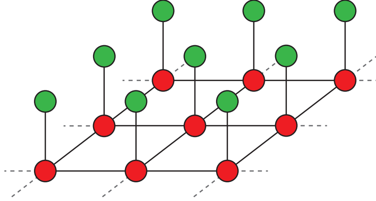
Figure 3.2: An MRF that is used for image denoising. The green nodes represent the observed, noisy pixels, while the red ones denote the restored, noise free pixels.
