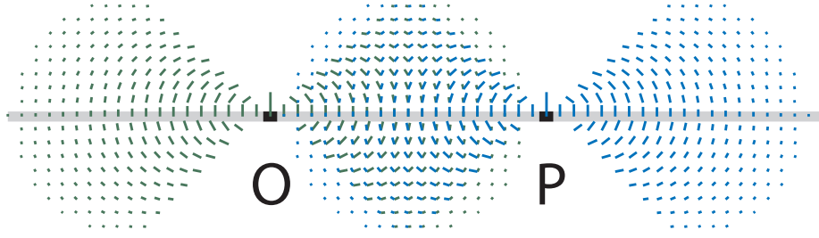
Figure 3.16: Voting fields of two tensors located at O and P . The tensors belong to the same structure, namely the gray line that should be restored. A tensor that receives votes by O and P accumulates the votes by simply summing them up. It is notable that from the subset of tensors, which receive two votes, only tensors located at the straight line are still stick tensors after the voting process. Hence the connecting line is the most likely connection.
