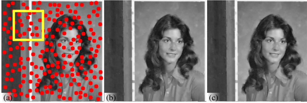
Figure 4.7: Inpainting of the circle mask, shown in (a). (b) Black initialization result: PSNR = 33.54 dB. (c) Mean initialization result: PSNR = 34.30 dB.
