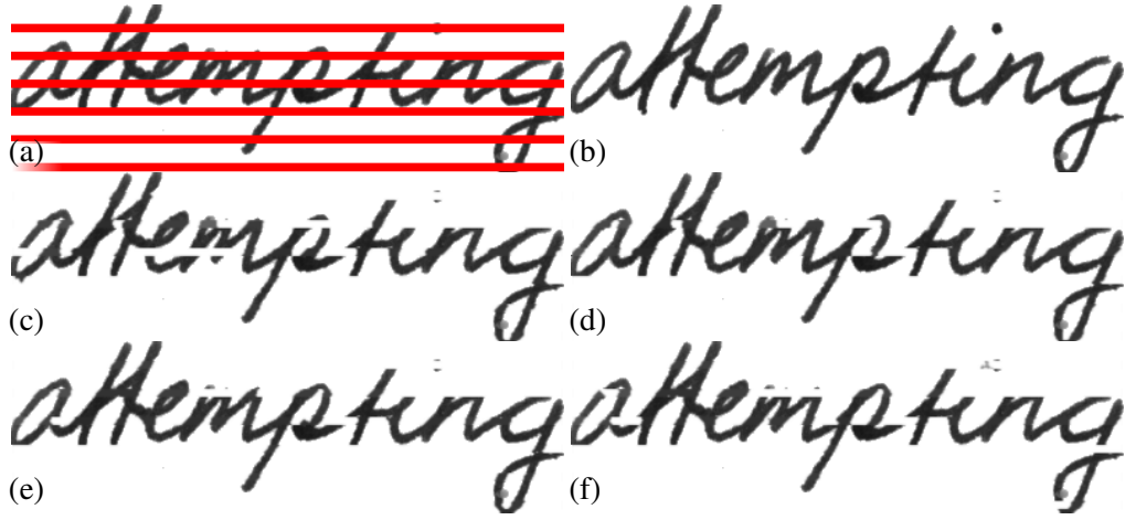
Figure 4.21: Impact of \sigma . (a) Input image with superimposed mask. The mask regions are 5 pixels wide. (b) Ground truth image. (c) \sigma = 3 : 14.83 dB. (d) \sigma = 5 : 15.83 dB. (e) \sigma = 9 : 16.14 dB. (f) \sigma = 12 : 15.03 dB.
