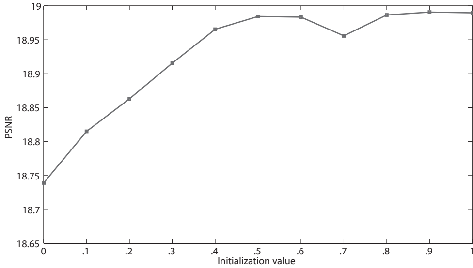
Figure 4.16: Evaluation of the initialization value.
