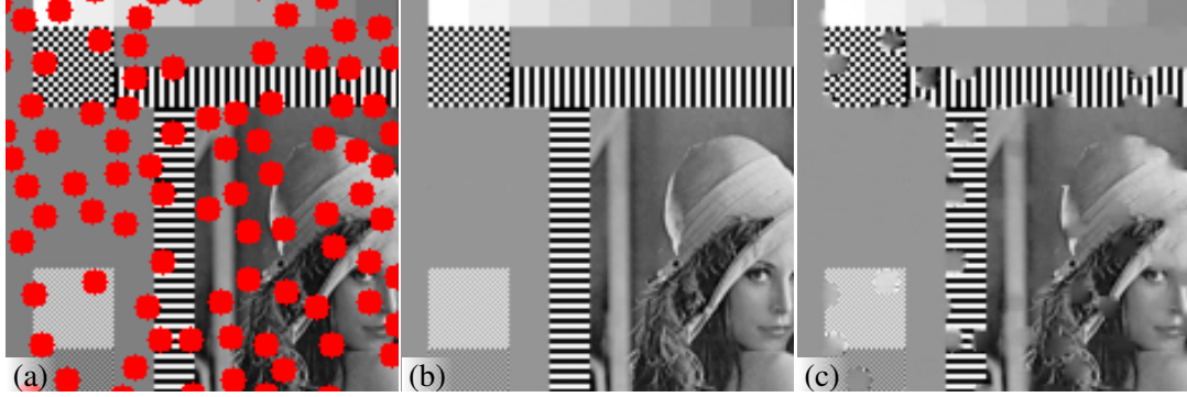
Figure 4.6: Limitation of the inpainting algorithm. (a) Input image. (b) Ground truth image. (c) Image inpainted with \eta = 110 . The PSNR value of the inpainting result is low, namely 24.93 dB.
