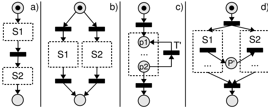
Figure 8: Petri Net Service Composition Patterns
