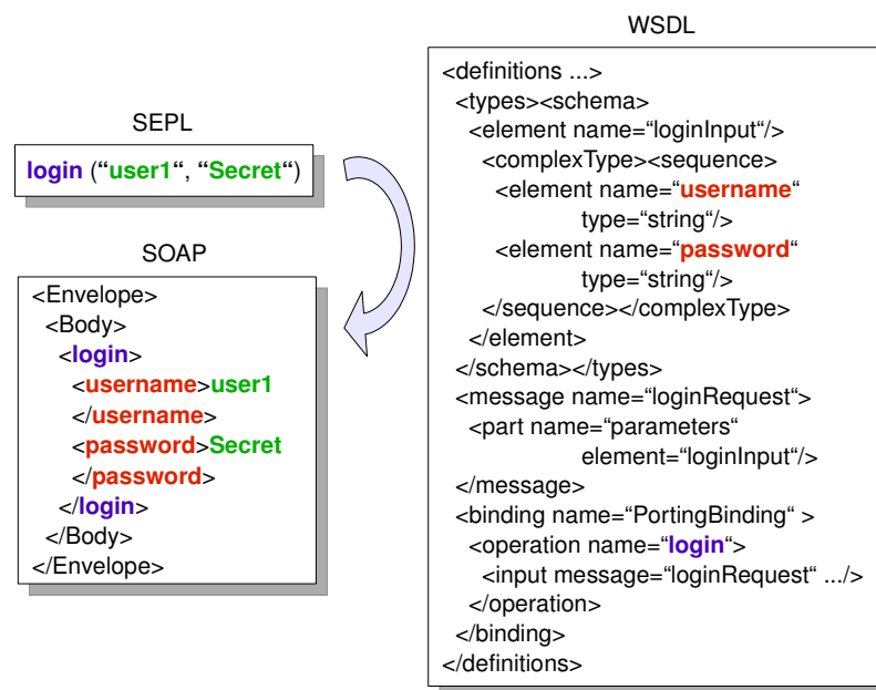
Figure 10: SEPL-to-SOAP Mapping
