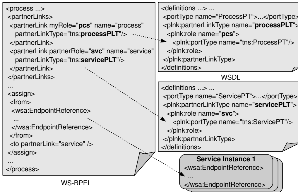
Figure 7: BPEL partnerLink Mapping
