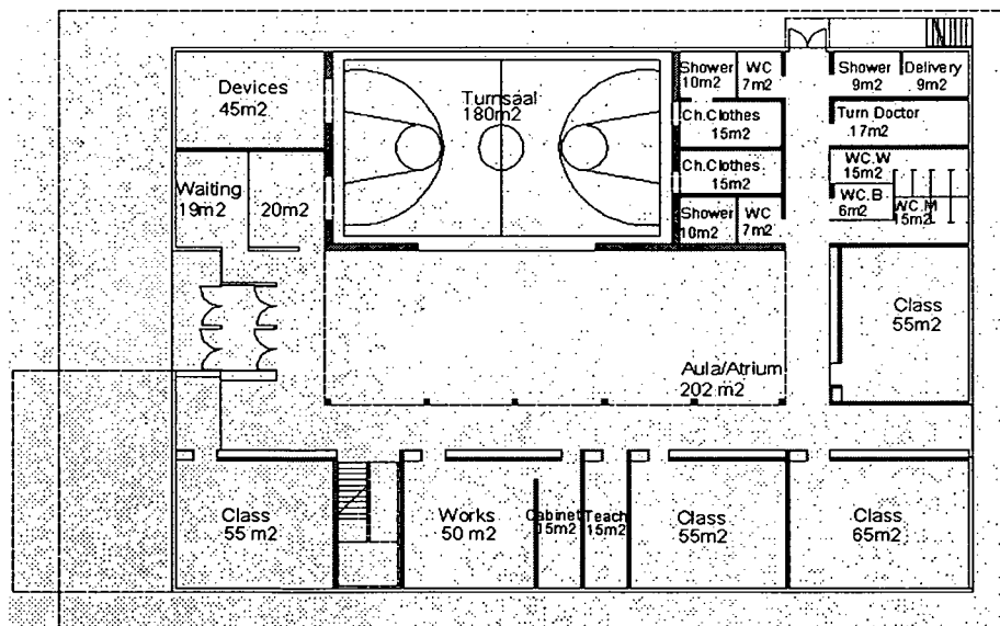
Figure A.19. Ground floor plan project_6
