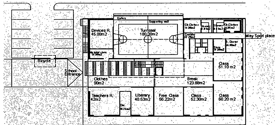
Figure A.13. Ground floor project_4
