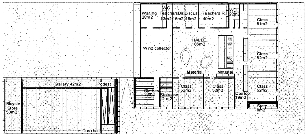
Figure A.10. Ground floor plan project_3
