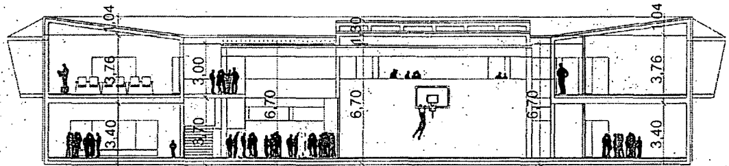
Figure A.6. Section project_2
