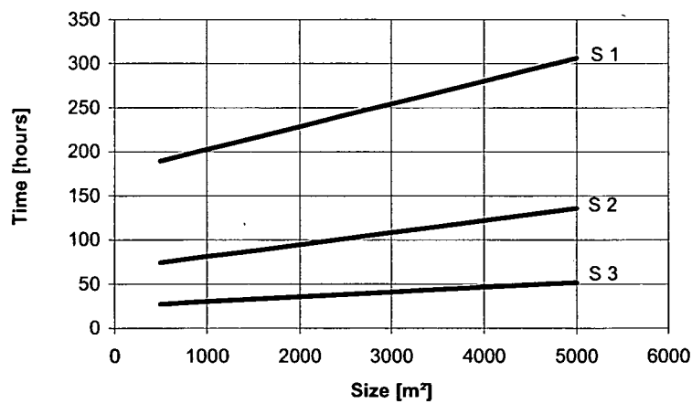
Figure 7. Illustrative examples of time requirements as a function of project size for three different simulation studies (scenarios 1 to 3 as per table 18)
