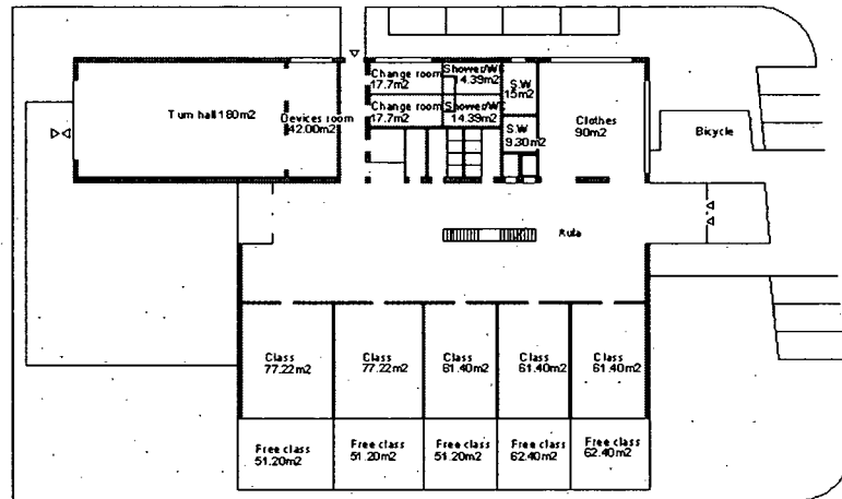
Figure A.4. Ground floor plan project_1
